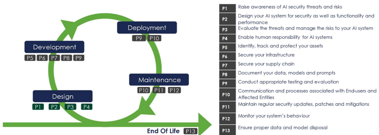
Figure 4.1-1: AI Lifecycle
